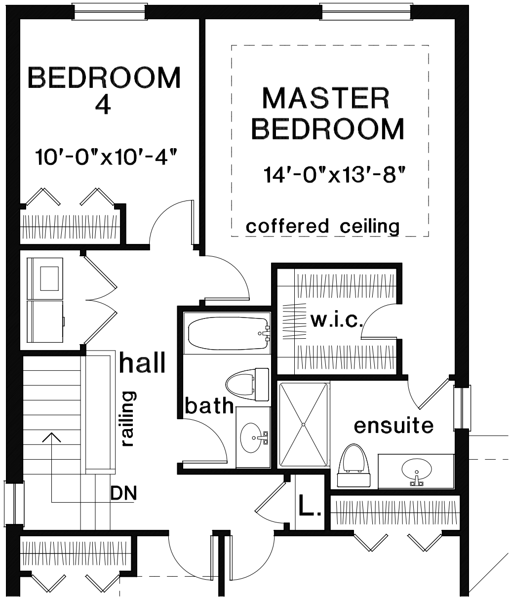
second floor 4 bed
