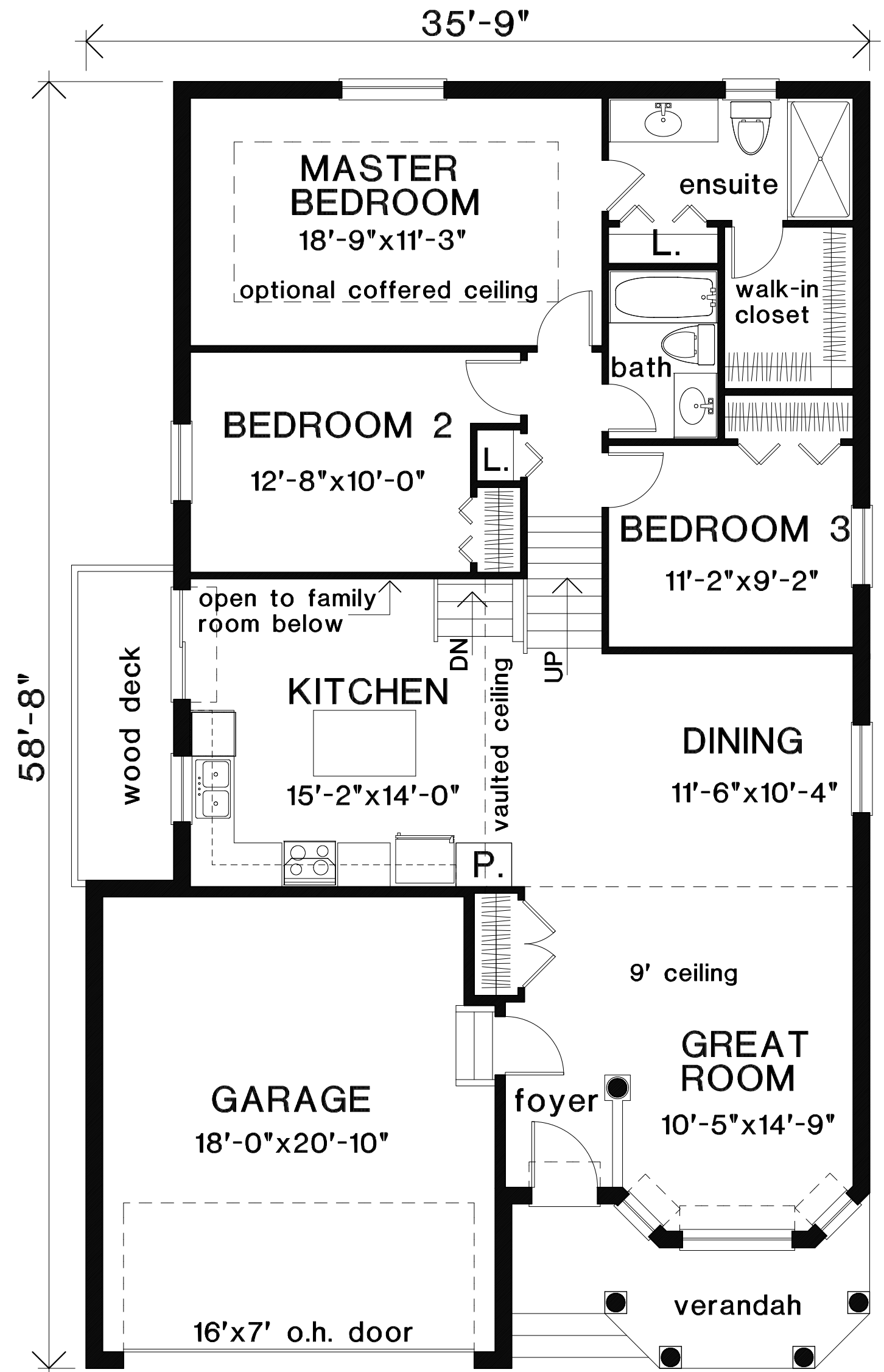
Plan A
